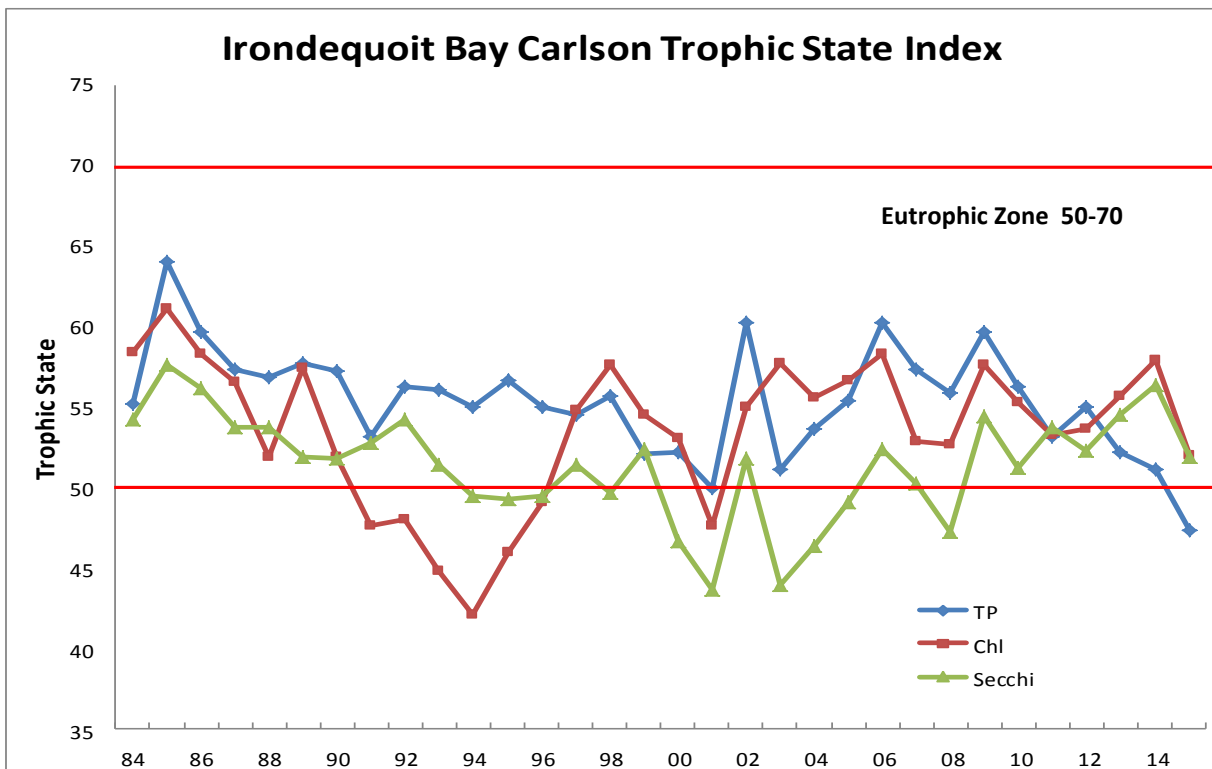
Figure 24 Trophic State Index scores for total phosphorus, chlorophyll-a and Secchi disk 1981-2015 using summer mean concentrations.
