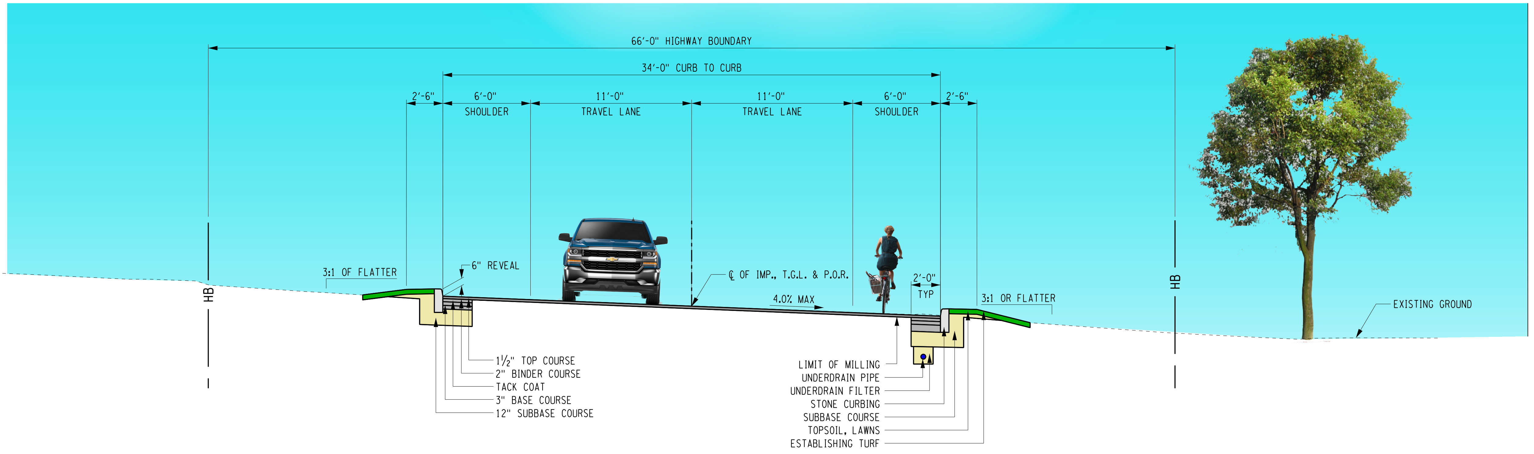
HINCHEY ROAD (COUNTY ROAD 237) TYPICAL SECTION - SUPERELEVATED
