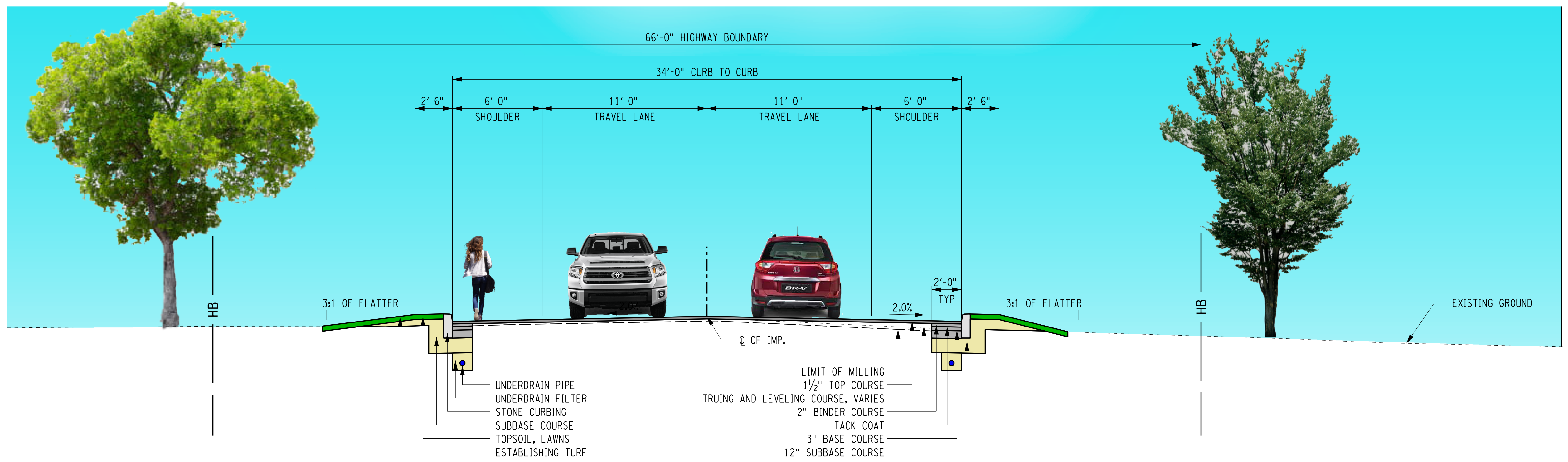
HINCHEY ROAD (COUNTY ROAD 237) TYPICAL SECTION - NORMAL CROWN
