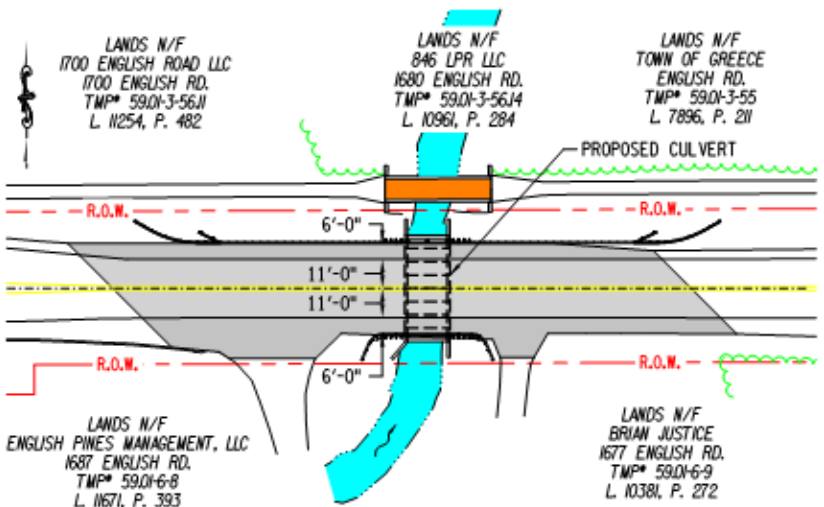
ENGLISH ROAD CULVERT PLAN 600 FEET EAST OF LONG POND ROAD NOT TO SCALE
