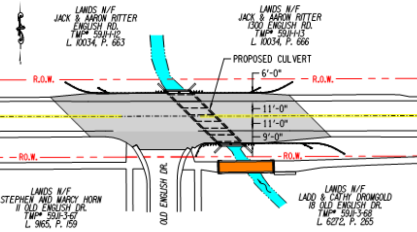
ENGLISH ROAD CULVERT PLAN AT OLD ENGLISH DRIVE NOT TO SCALE
