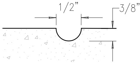
SECTION A-A (TYPICAL NUMBER CROSS SECTION)
