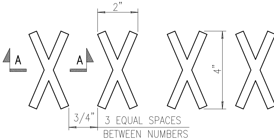
SECTION A-A (TYPICAL NUMBER CROSS SECTION)
