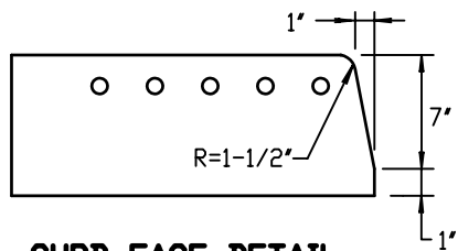
CURB FACE DETAIL
