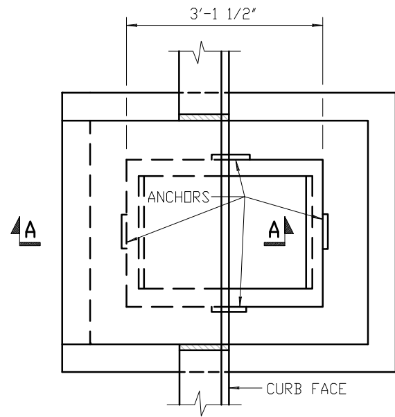
PLAN FOR PIPE GREATER THAN 18" UP TO 24"
