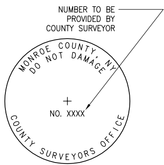
GEODETIC MONUMENT CAP INSCRIPTION N.T.S.
