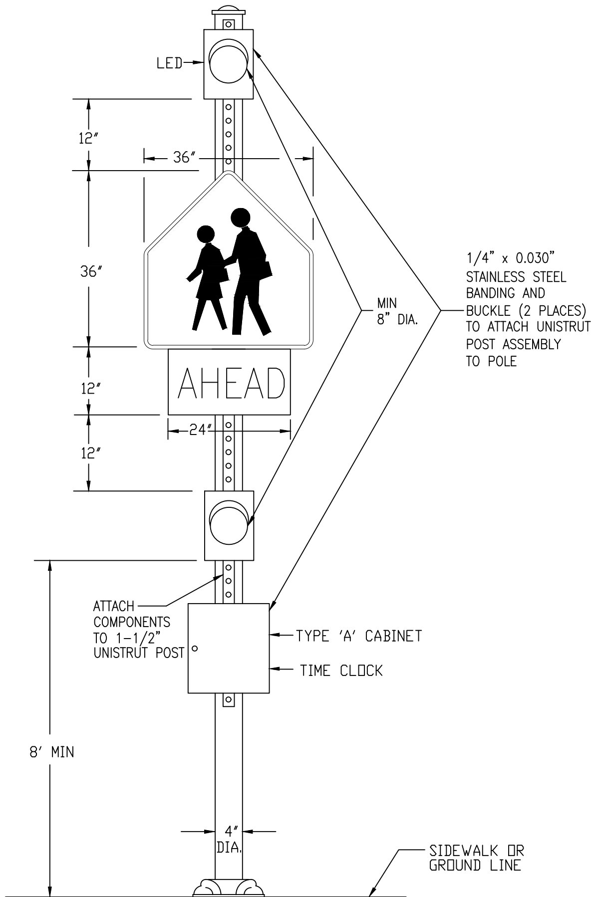
ADVANCE SCHOOL ZONE WARNING FLASHER CONFIGURATION
