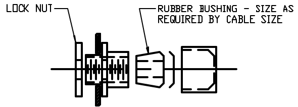
WIRE ENTRANCE CONDULET WITH LOCK NUT & RUBBER BUSHING, TYPE AB
